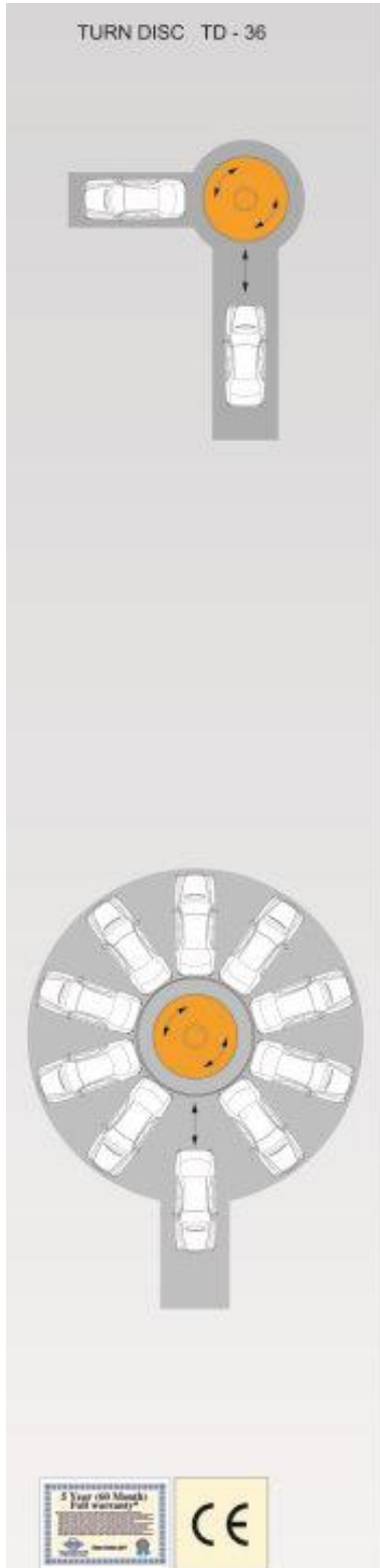
TD - 36 / A Installation on the floor
